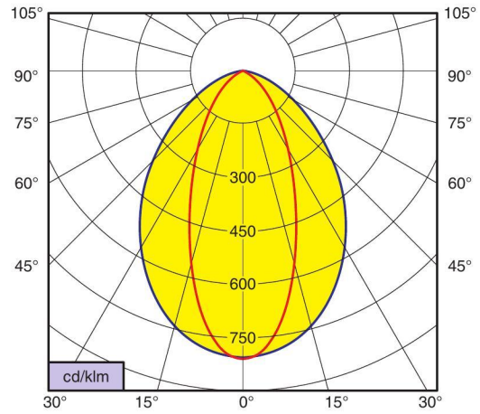
Figure 2 Luminous intensity distribution (LID) (red line: C0 - C180, blue line: C90 - C270)
